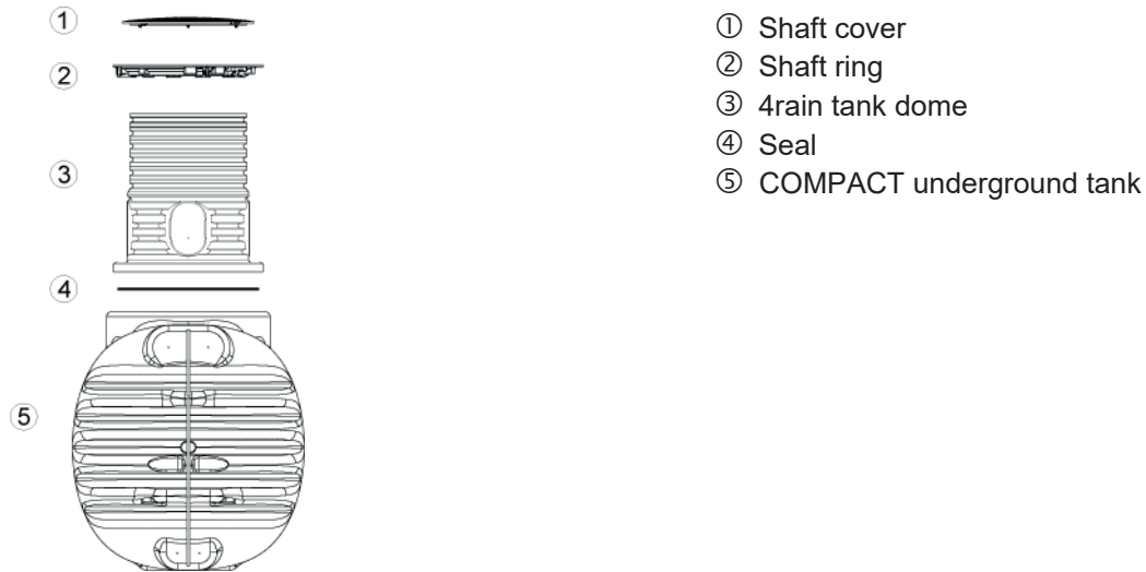
Fig. 19: Components – COMPACT
