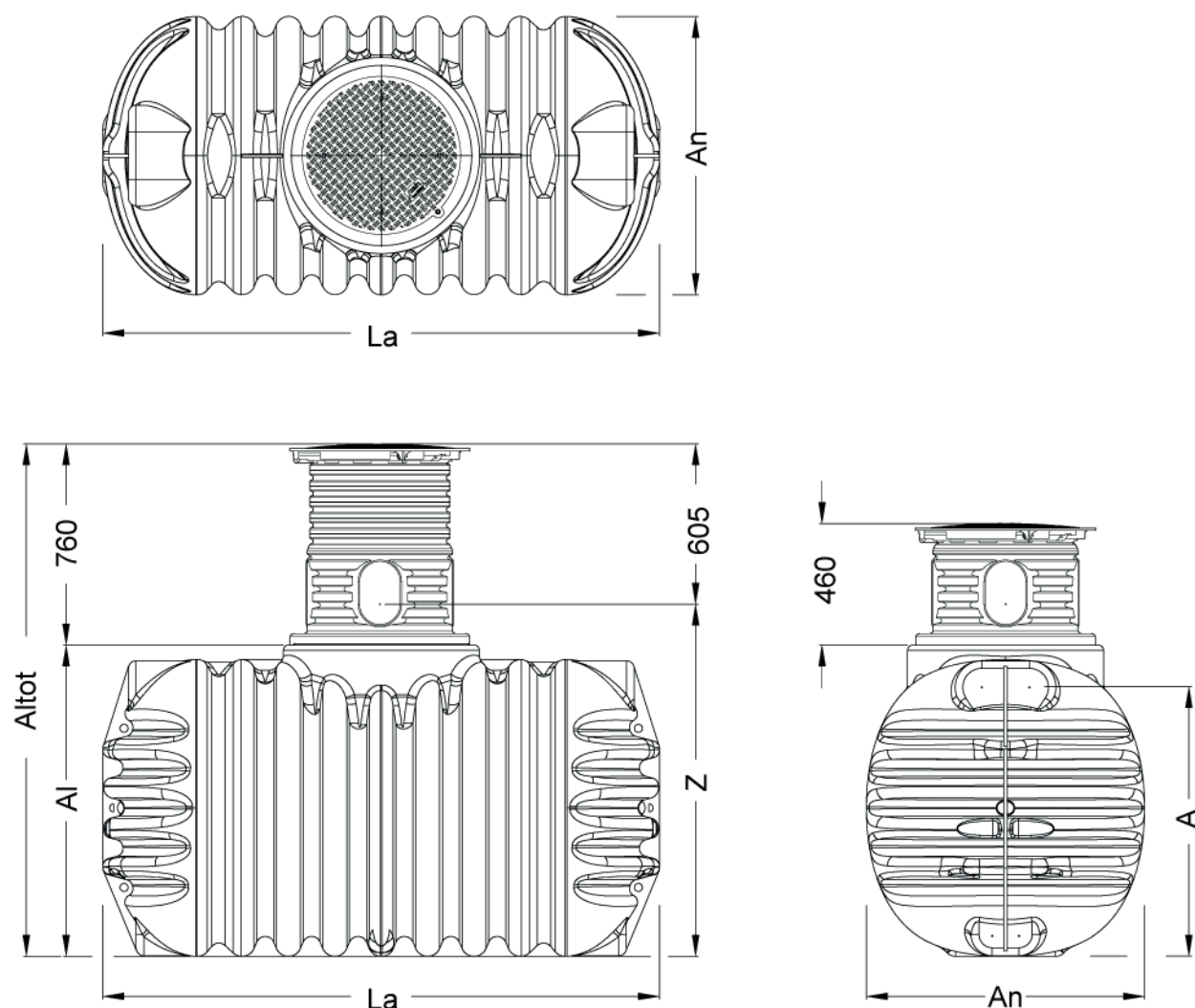
Fig.9: Dimensiones – COMPACT
