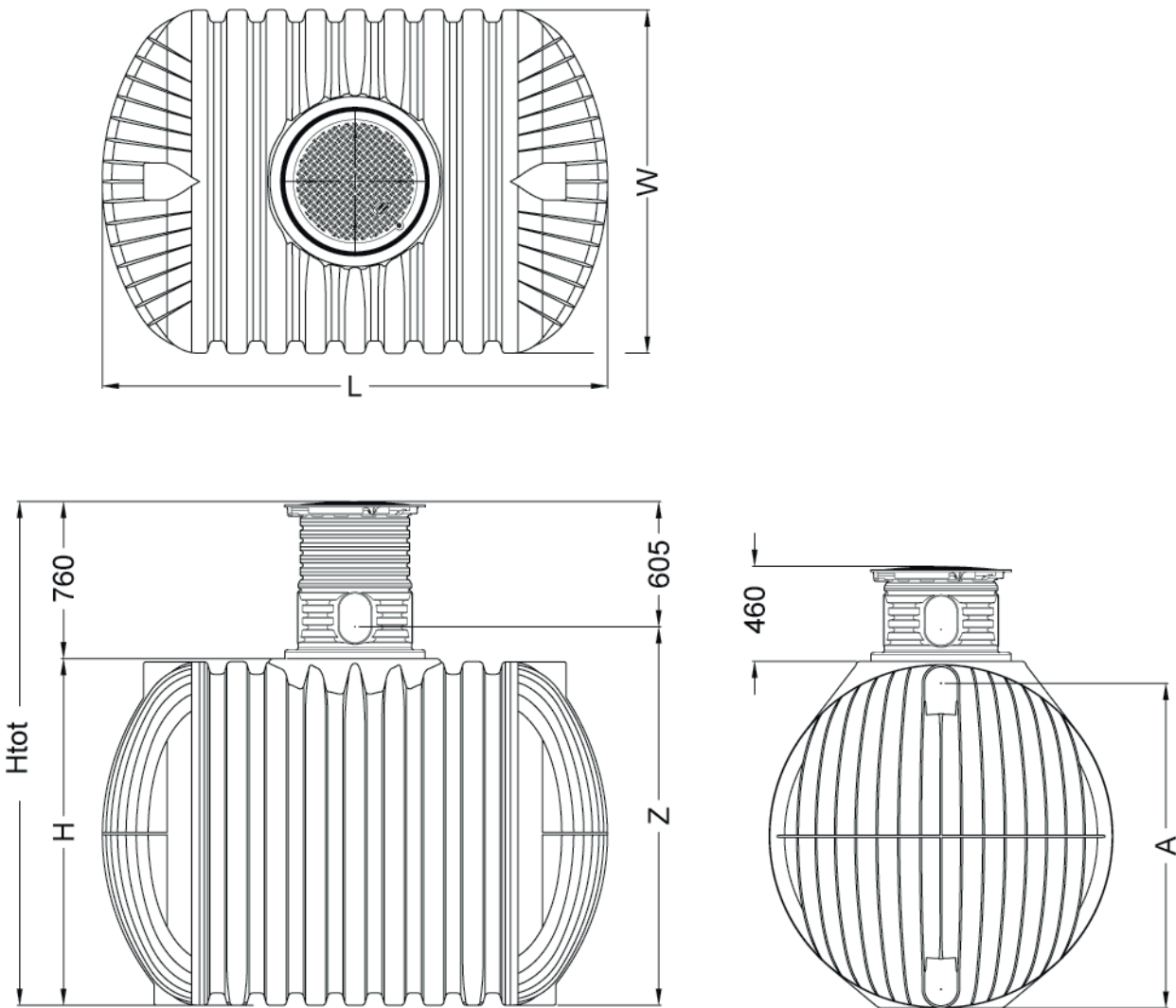
Fig. 10: Measurements – PROFI
