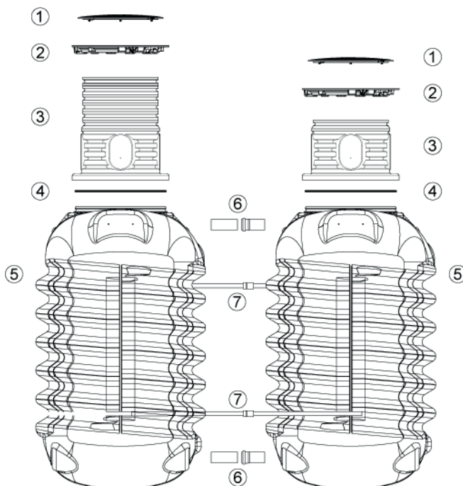
Fig. 18: Components – MODULARIS
